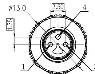
孔位示意图(3芯) HOLES ARRANGEMENT (3CORE)
