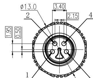
孔位示意图(4芯) HOLES ARRANGEMENT (4CORE)
