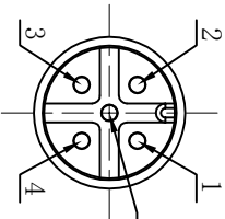
孔位示意图 (5芯) HOLES ARRANGEMENT (5CORE)
